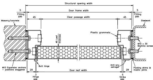
Fixing method
