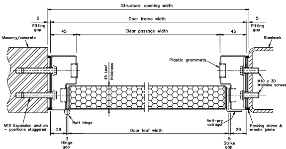
Sunray Single ExcluDoor® 5
